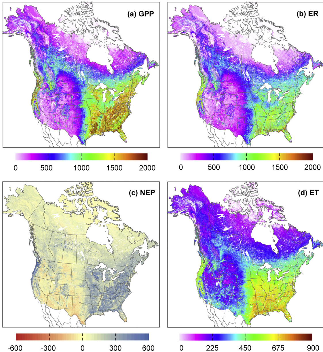
Fig. 3. Mean annual carbon and water fluxes over North America for the period 2001–2012: (a) GPP; (b) ER; (c) NEP; and (d) ET. The units for carbon fluxes are \text{g C m}^{-2} \text{ yr}^{-1} , and the units for ET are \text{mm yr}^{-1} .
