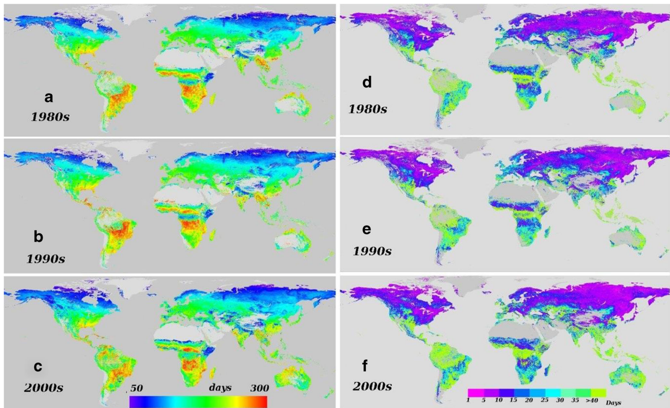
Fig. 7 Spatial pattern in average GSL ( a , b , and c ) and interannual standard deviation ( d , e , and f ). Note the first growing season is presented if there are multiple seasons within a year. Gray indicates no phenology detection
