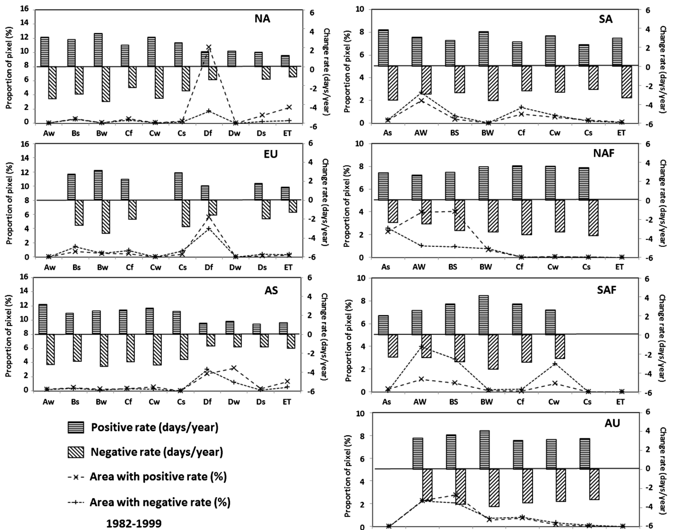
Fig. 9 The shift rate averaged from significant pixel-based trends ( P < 0.1 ) and the proportion of pixels with significant trends in growing seasonal length from 1982 to 1999
