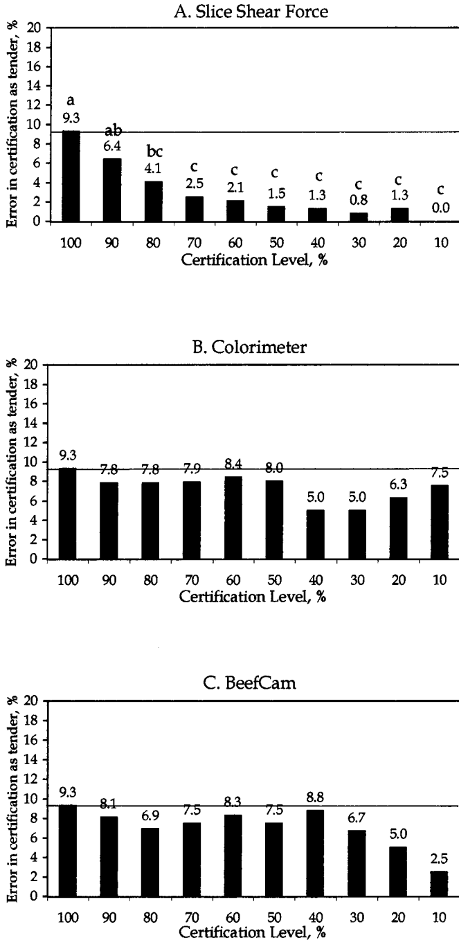
Figure 3. Error rates for certifying all carcasses as “tender” in increments of 10% of the sample (Phase II, n = 400 ). “Tender” was defined as longissimus Warner-Bratzler shear force of < 5 kg at 14 d postmortem. 100% certification means no tenderness sorting. a,b,c,d Means across certification levels within certification method lacking a common superscript letter differ ( P < 0.05 ).
