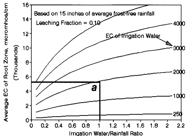
Figure 5. Relationships of average root zone and irrigation water salinity and irrigation and rainfall depths.
