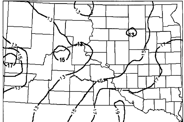
Figure 4. Average normal growing season precipitation in South Dakota (April 1 - October 31) for 1961-1990.
