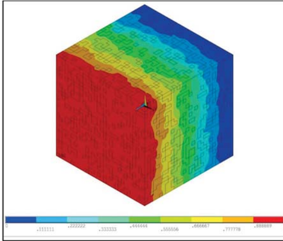
Figure 12. Electric potential distribution of model 2.
