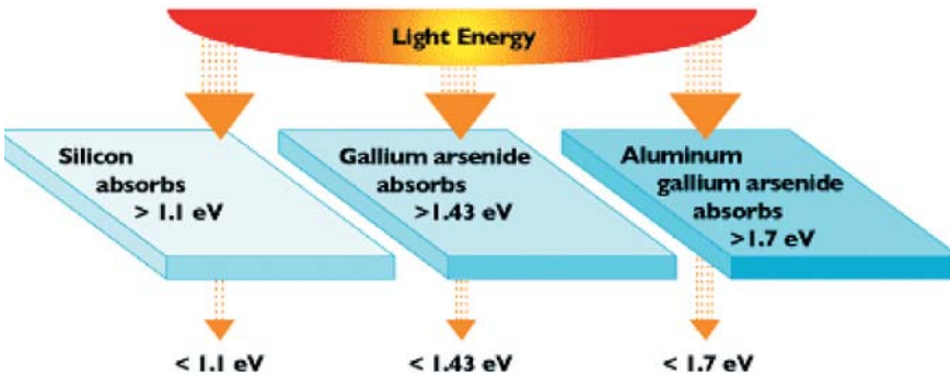
Figure 1. Band gap energies for silicon, gallium arsenide, and aluminum gallium arsenide.
