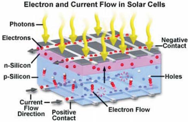
Figure 4. Photovoltaic process.
