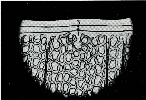
Fig. 11. Cross section (magnified 50 times) showing how a three-coat paint job anchors to the cellular structure of wood.
