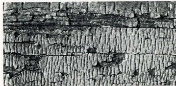
Fig. 13. Investigation of the formula before buying would avoid such results as these. Usually hard-type paints composed of cheap extenders and linseed oil substitutes fail like this.
