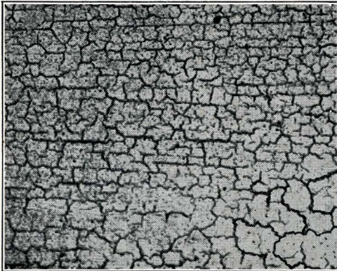
Fig. 44. Alligatoring.
