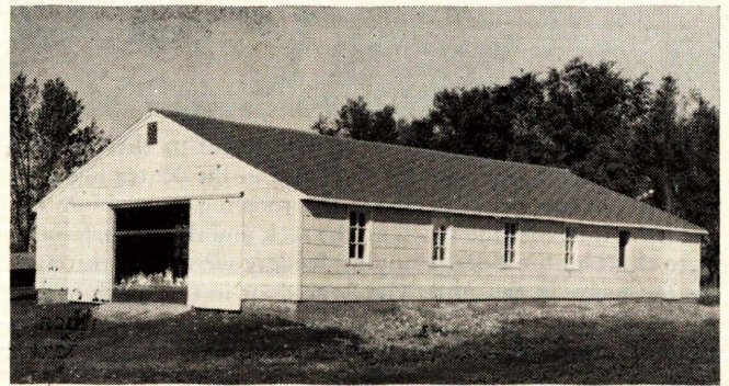
Fig. 8. This is one of the modern insulated and ventilated poultry houses built from S. D. Extension Circular No. 515. The house is 30 x 50 feet and will accommodate 500 to 600 laying hens.
