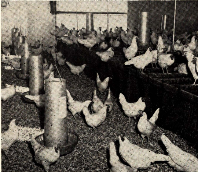
Fig. 9. Note the arrangement of equipment in this modern poultry house. The dropping pit island in the center has both feed and water installed above the roosting area. Note the welded wire under the roosts on the rack and the 1/4-inch hardware cloth on the sides. Hanging feeders were used throughout the house in this unit. The large door in the south end of the house admits sun and air in the summer and is a handy clean-out door. Small tractors and equipment can enter through this door.
