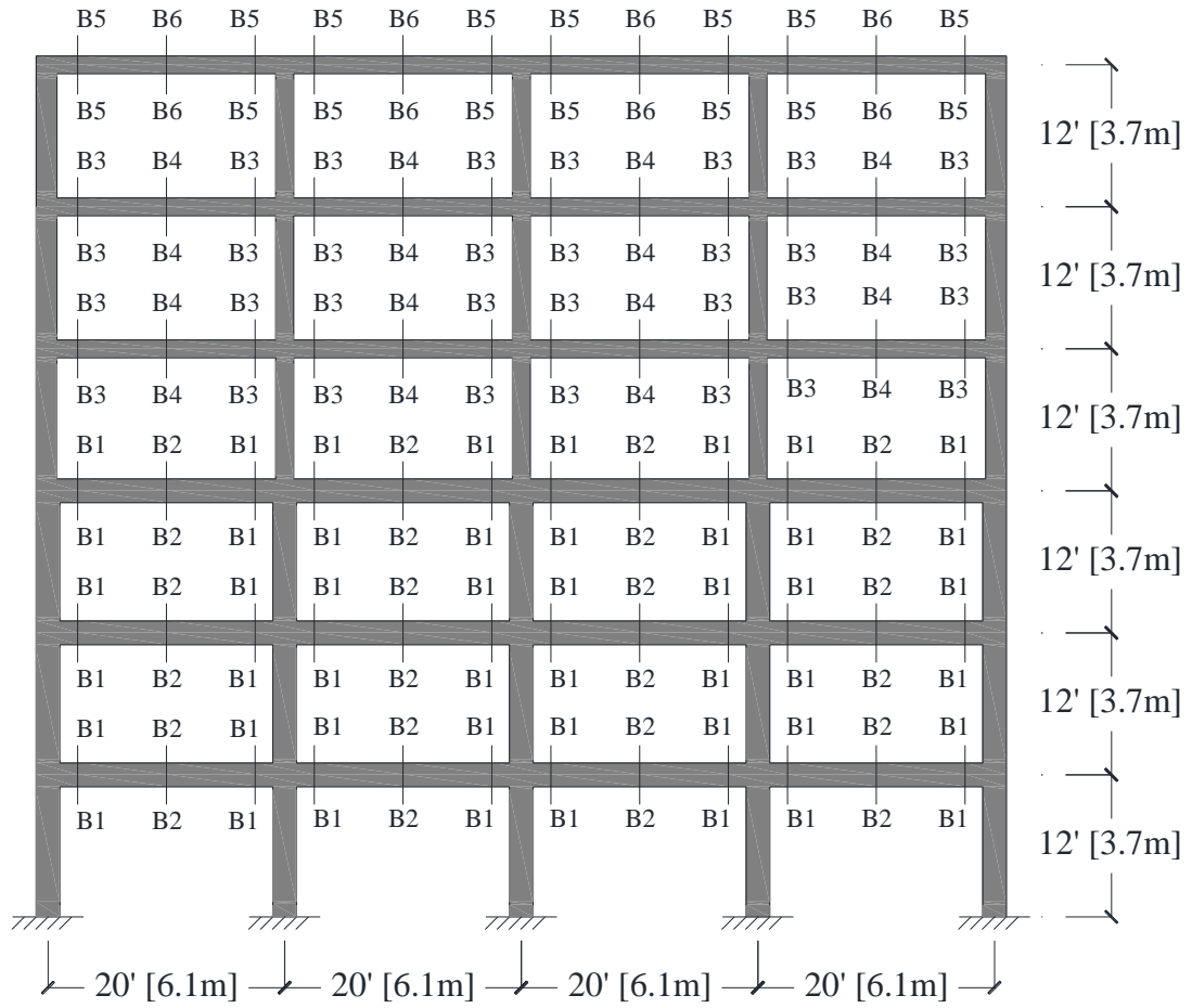
Figure 4.9- Six-Story Ordinary Moment-Resisting Frame
