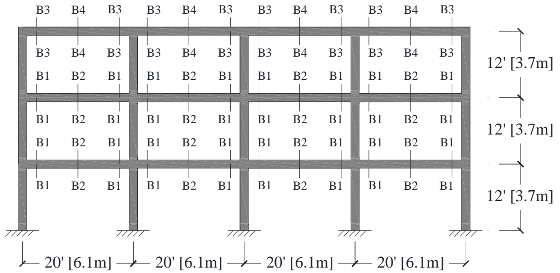
Figure 4.3- Three-Story Ordinary Moment-Resisting Frame
