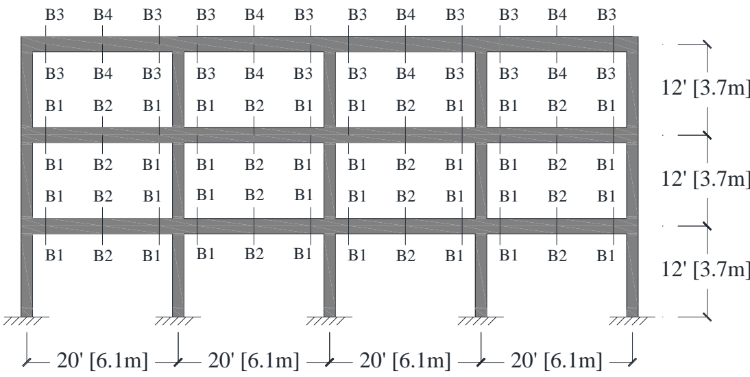
Figure 4.5- Three-Story Intermediate Moment-Resisting Frame
