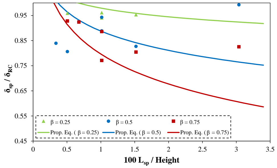
Figure 5.14- Summary of Results for IMRFs
