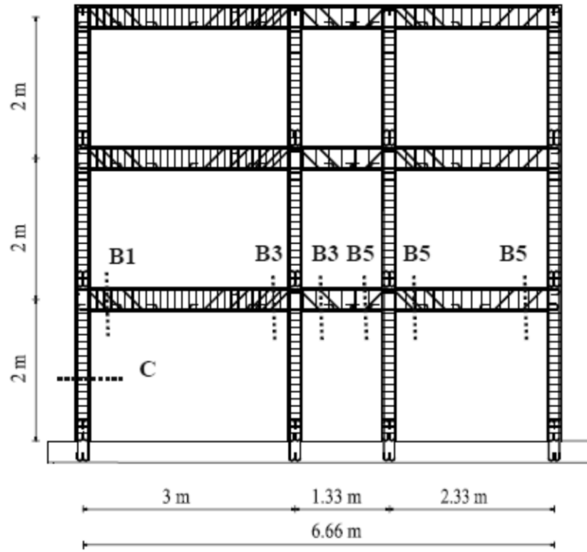
Figure 2.19- Gravity Frame Tested by Calvi et al. (2001)
