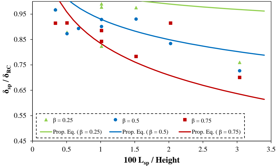
Figure 5.15- Summary of Results for OMRFs
